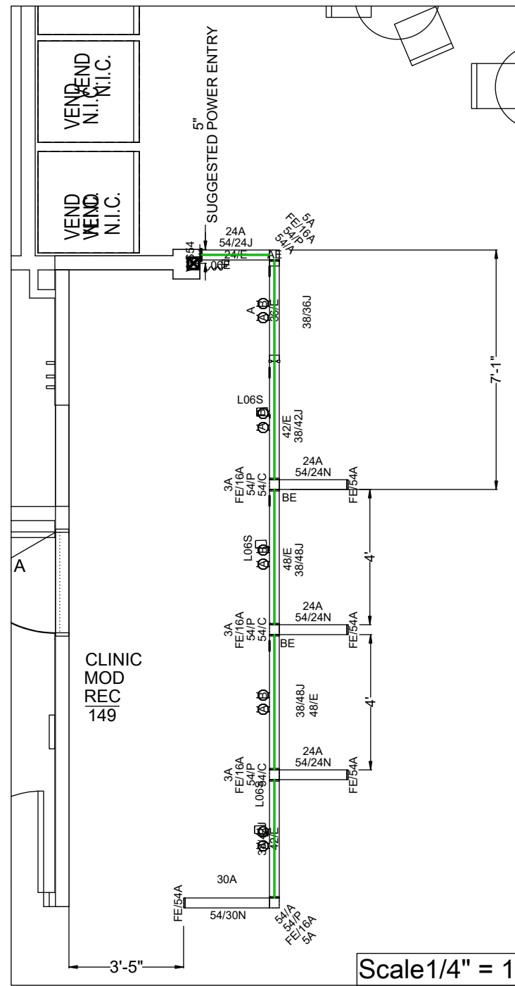
ELECTRICAL PLAN CLINIC MOD REC 149
