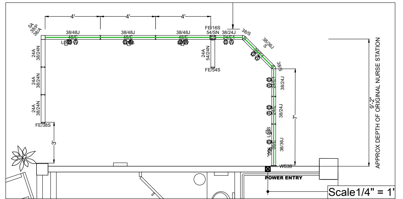
ELECTRICAL PLAN REGISTRATION 102
