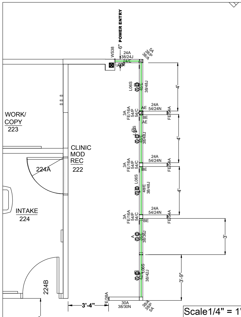
ELECTRICAL PLAN CLINIC MOD REC 222
