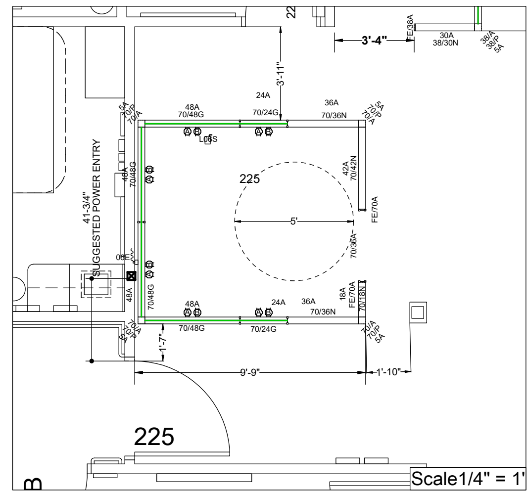
ELECTRICAL PLAN CBOC AREA 225
